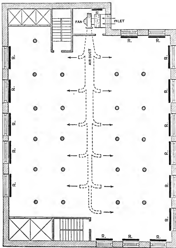
FIG. 9. A SCHEME FREQUENTLY USED IN LOFT BUILDINGS DEVOTED TO LIGHT MANUFACTURING
